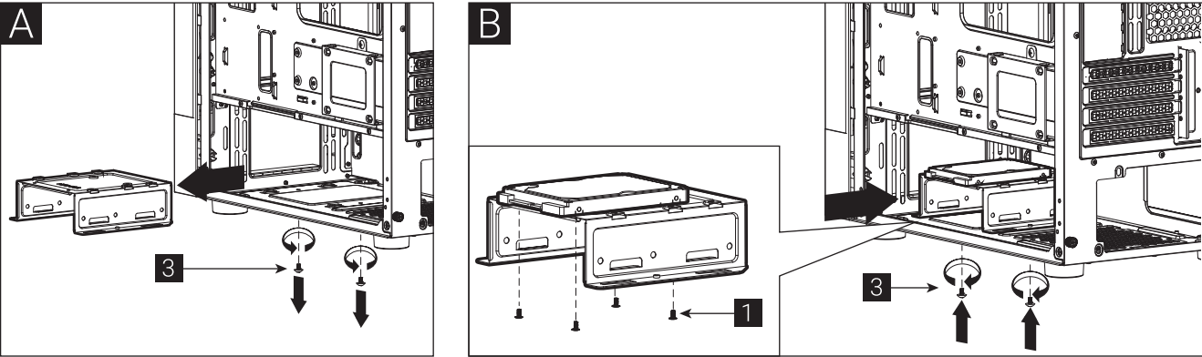
(5b) Install 2.5" SSD x 1
