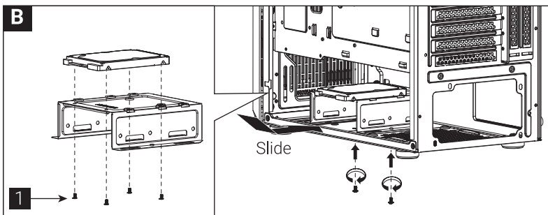
(5b) Install 3.5" HDD x1
