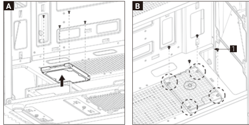
(5b) Install 2.5" SSD x1
