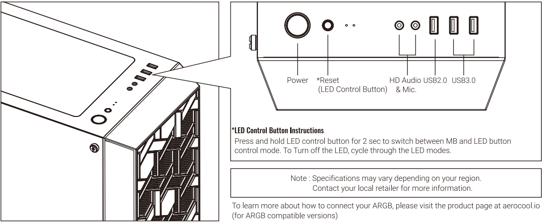
I/O Panel
