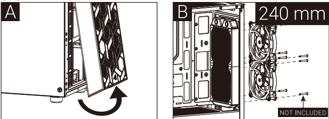
(6b) Install Front Radiator
