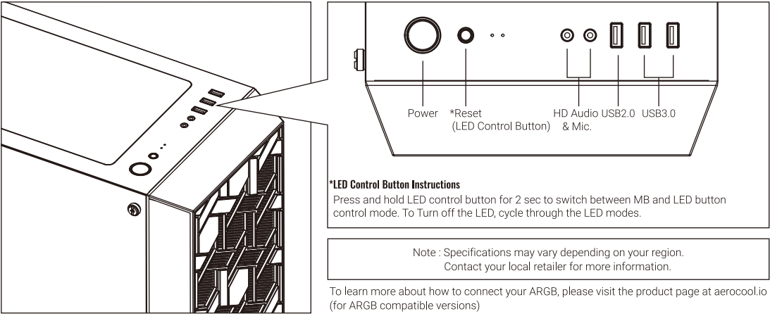
I/O Panel
