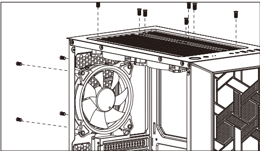
(7b) Install Rear and Top Fan
