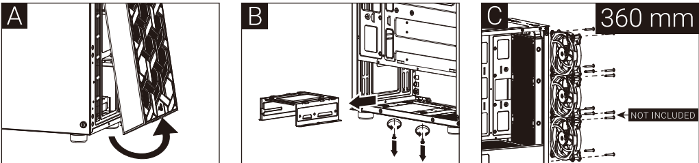
(6b) Install Front Radiator
