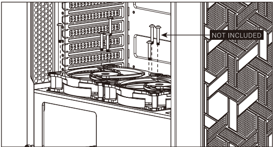
(7c) Install PSU Fans
