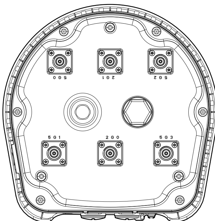
Figure 7 AP-574 Bottom View (without Aesthetic Cover)
