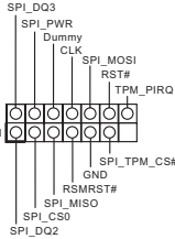
SPI_TPM_J1
