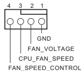
CPU_FAN2/WP
