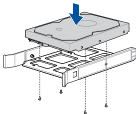
3.5" Drive
