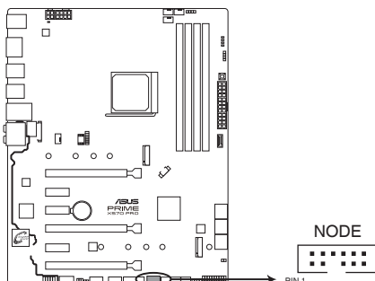
PRIME X570-PRO Node connector
