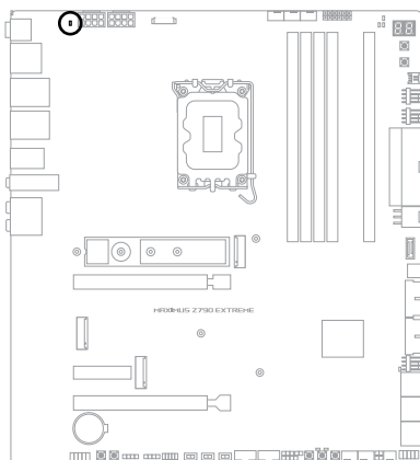
□ PLUG_8PIN_PWR
