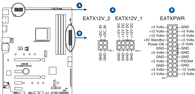
TUF GAMING X570-PLUS ATX power connectors
