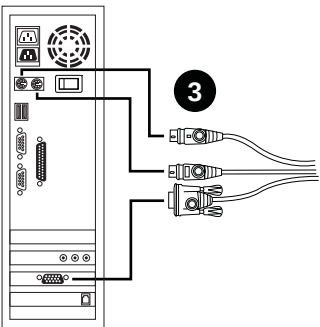
PS/2 KVM Cable Connection
