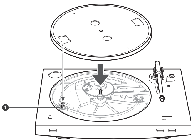
1 Motor pulley (brass-colored)
