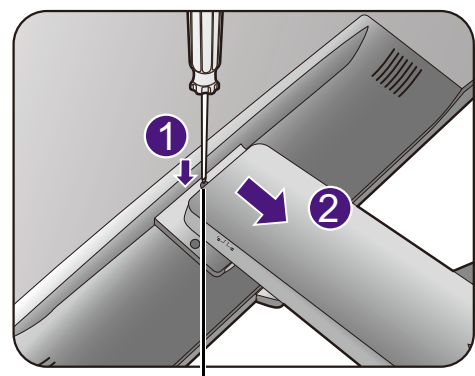
Release button
