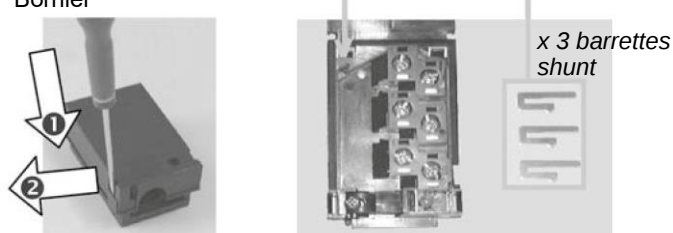
Bornier
