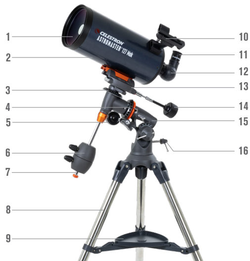
(in figura AstroMaster 127EQ MAK)
