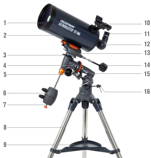
(Mostrado AstroMaster 127EQ MAK)
