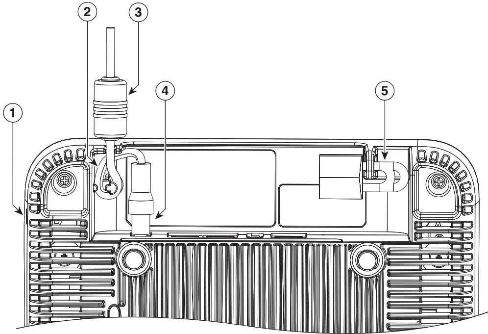
Figure 4 Routing the DC Power Cable
