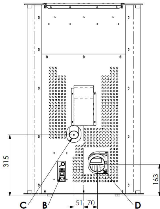
AURORA pellet stove dimensions
