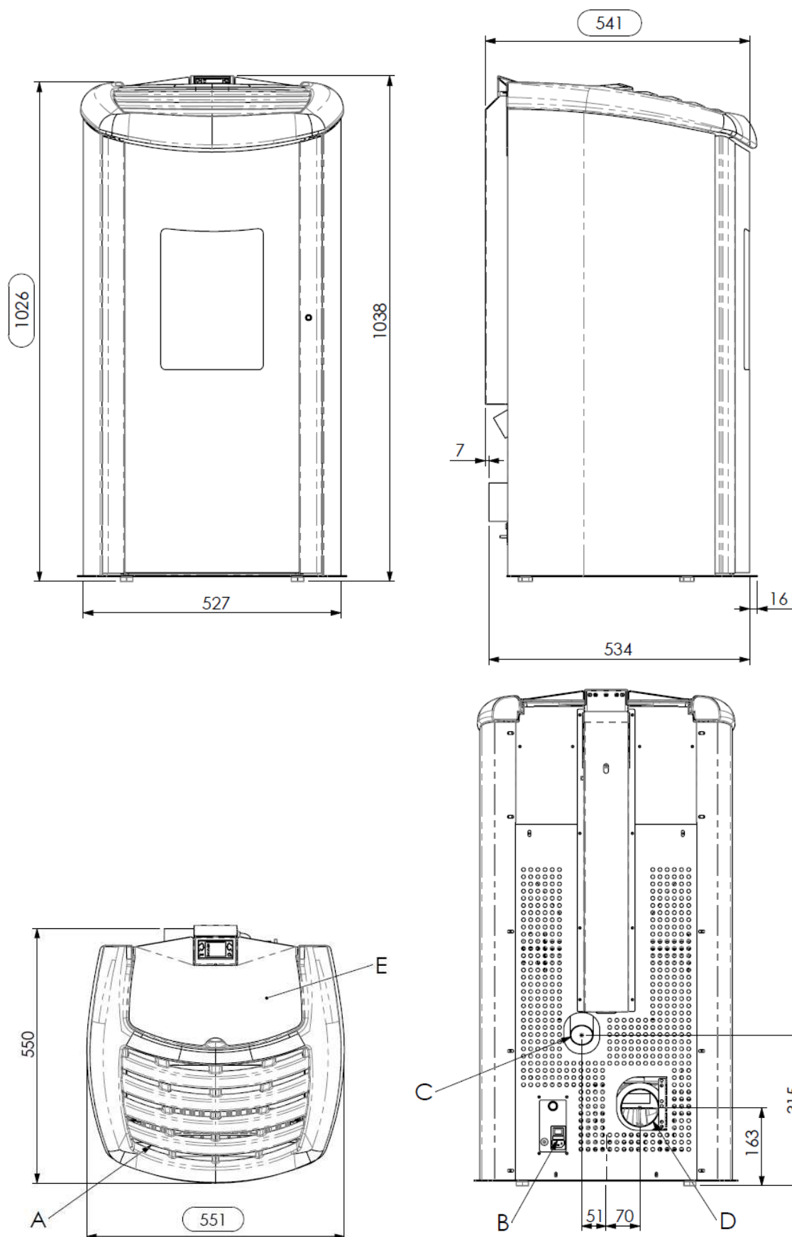
DIAMOND pellet stove dimensions
