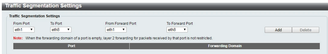
Figure 4.46 – Security > Traffic Segmentation
