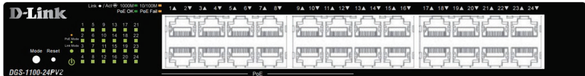
Figure 2-5 – DGS-1100-24PV2 Front Panel
