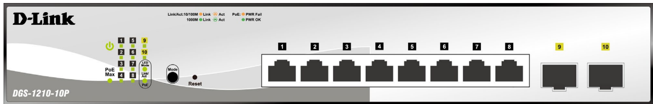
Figure 1.3 – DGS-1210-10P Front Panel
