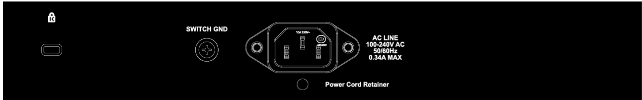
Figure 1.8 – DGS-1210-20 Rear Panel
