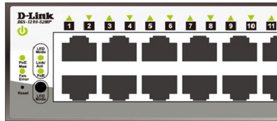
Figure 1.21 –LED Indicators on DGS-1210 series
