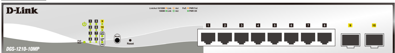
Figure 1.5 – DGS-1210-10MP Front Panel
