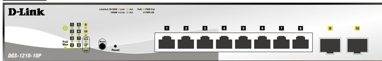
Figure 1.3 – DGS-1210-10P Front Panel
