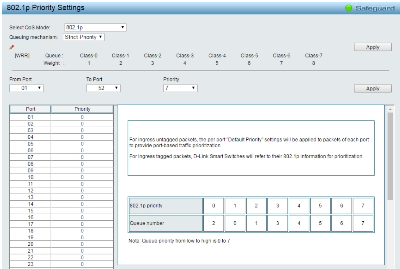
Figure 4.96 – QoS > 802.1p/DSCP/ToS
