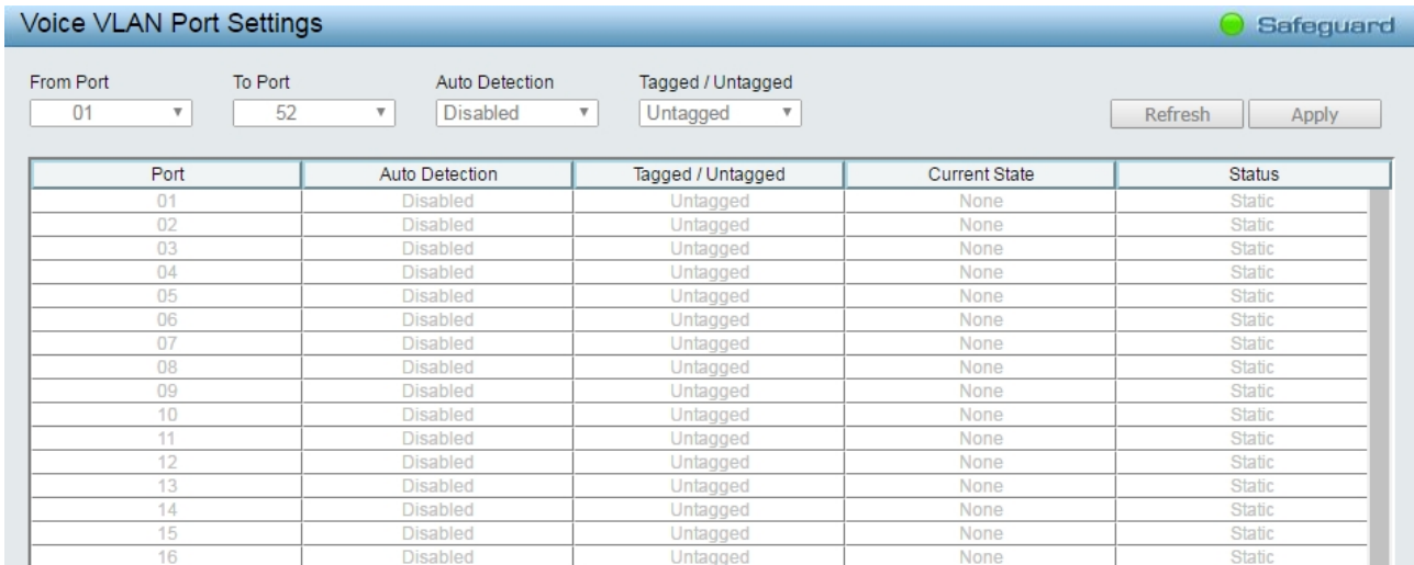
Figure 4.46 – VLAN > Voice VLAN > Voice VLAN Port Settings
