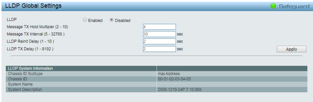
Figure 4.70 – L2 Functions > LLDP > LLDP Global Settings
