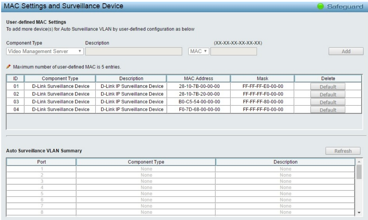
Figure 4.49 – VLAN > Auto Surveillance VLAN > MAC Settings and Surveillance Device
