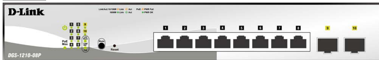
Figure 1.1 – DGS-1210-08P Front Panel
