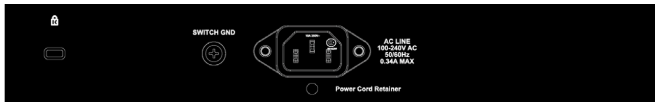
Figure 1.4 – DGS-1210-16 Rear Panel
