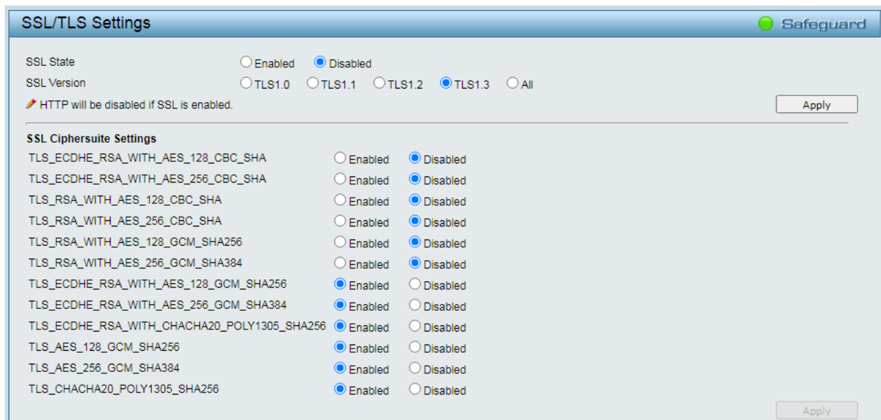
Figure 4.116 – Security > SSL/TLS
