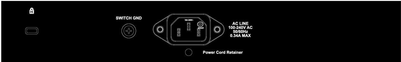
Figure 1.8 – DGS-1210-20 Rear Panel
