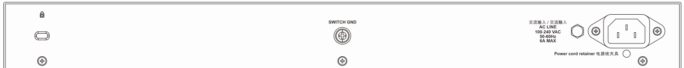
Figure 1-12 Rear panel view of the DGS-1250-52XMP
