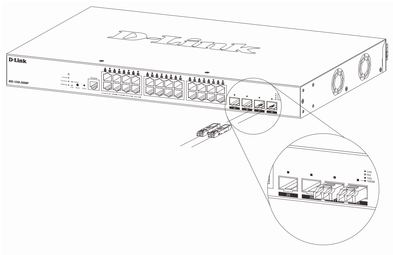
Figure 2-4 Inserting transceivers into the transceiver ports
