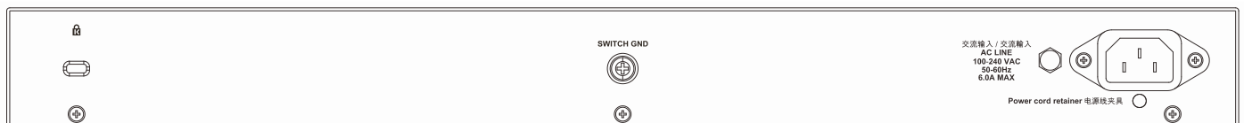
Figure 1-10 Rear panel view of the DGS-1250-28XMP
