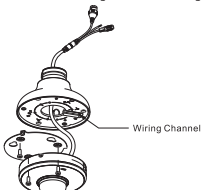
Figure 4-4 Installing the mounting plate
