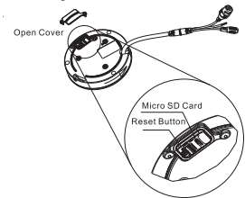
Figure 2-3 Reset button
