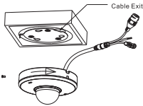
Figure 3-5 Rotating the speed dome pedestal
