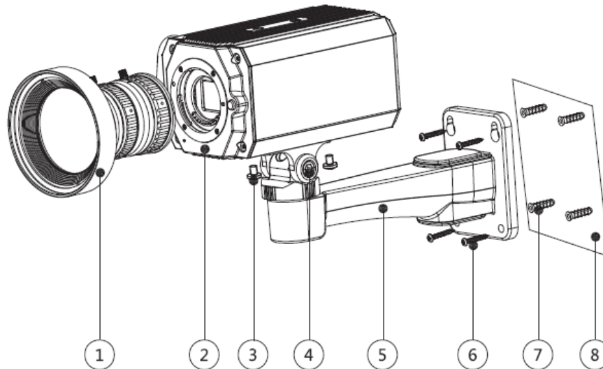
Figure 9-6 Device components
