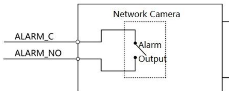
Figure 1-4 Alarm output
