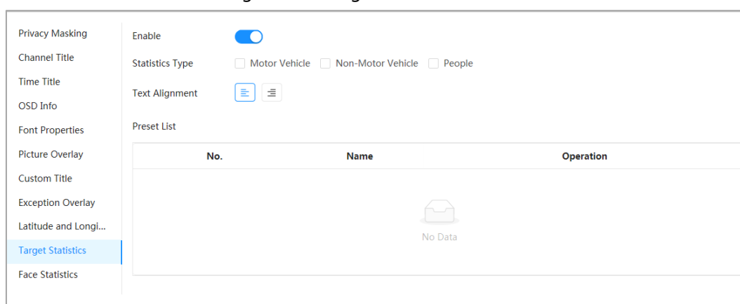
Figure 4-25 Target statistics
