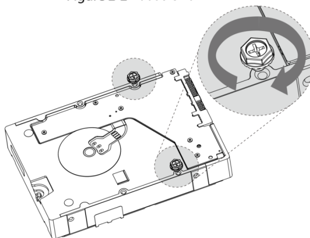
Figure 2-2 Put screws
