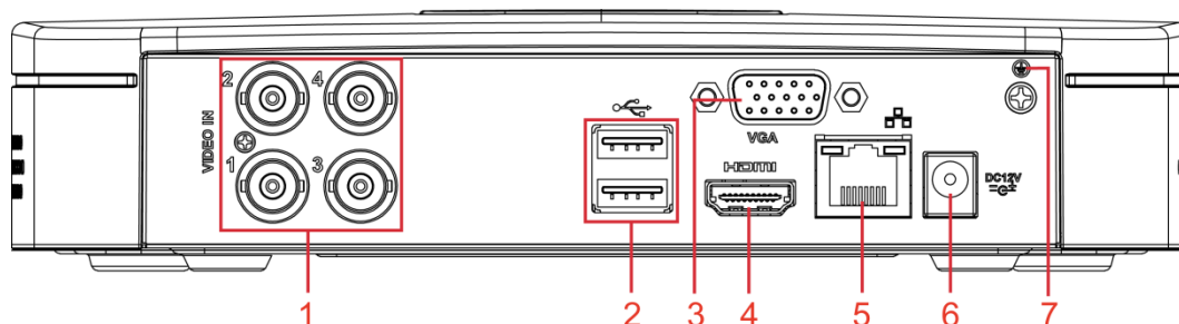
Figure 3-20 Rear panel
