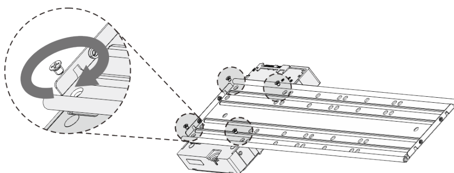
Figure 2-19 Fix HDD
