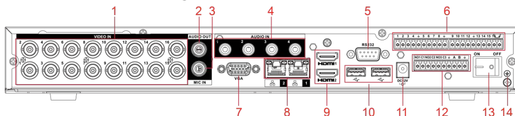
Figure 3-15 Rear panel
