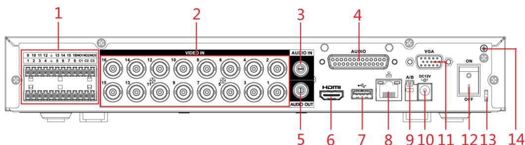
Figure 3-12 Rear panel
