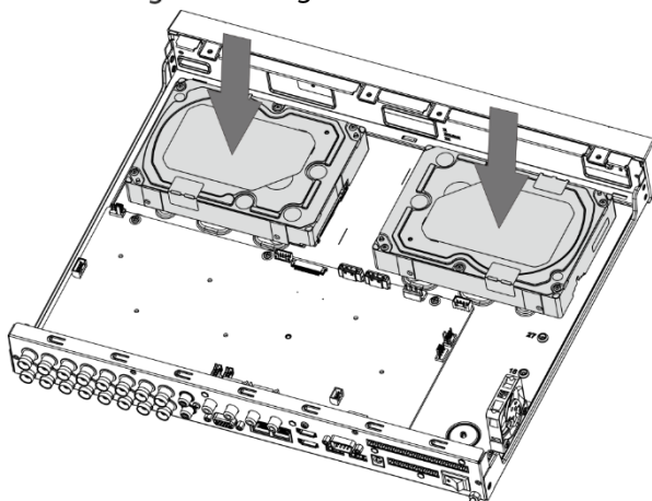
Figure 2-3 Align screws
