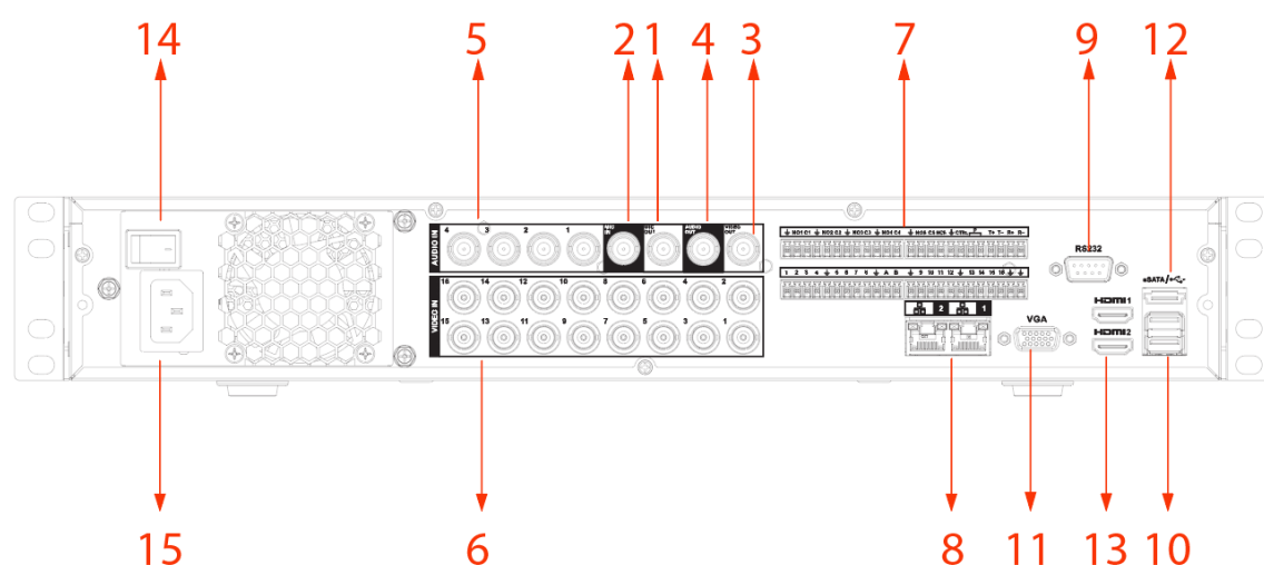
Figure 3-20 Rear panel (3)
