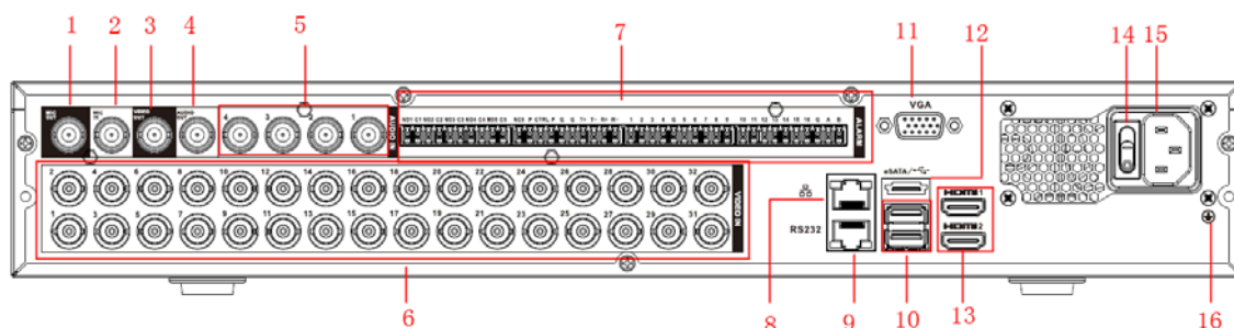
Figure 3-19 Rear panel (2)
