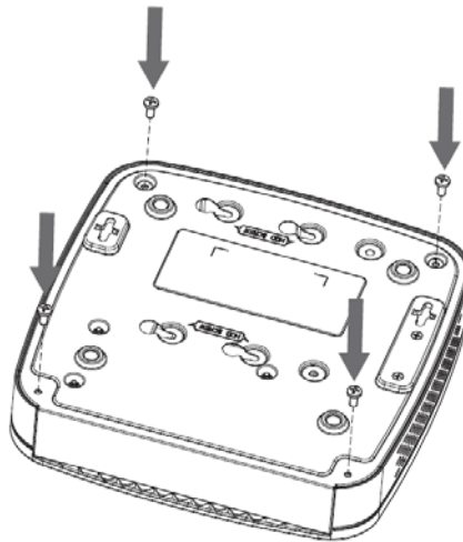
Figure 2-35 Fasten screws
