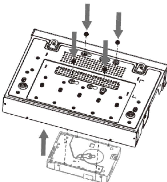
Figure 2-26 Fasten screws
