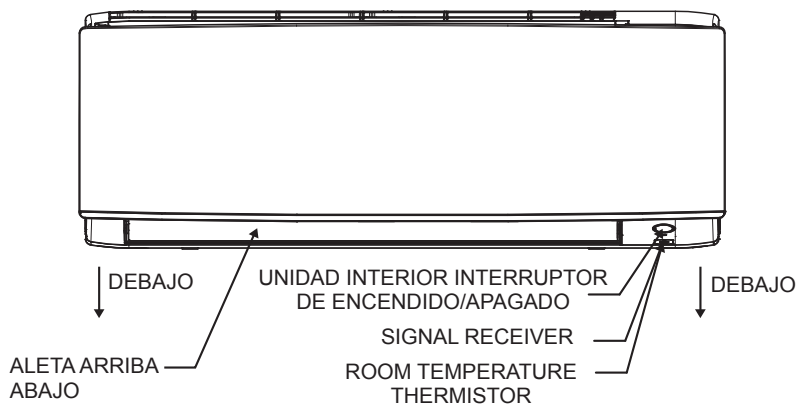
VISTA FRONTAL
