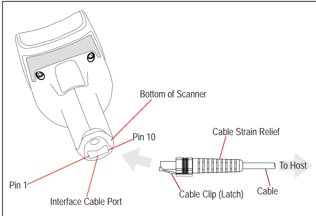
Figure 14. Standard Cable Pinouts: Handheld
