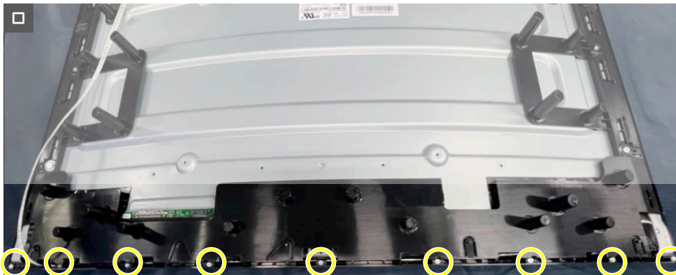
Figure 36. Removing the middle frame
