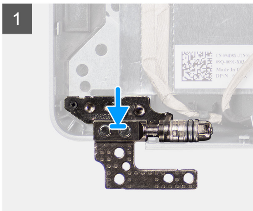
2x M2.5x3.5
