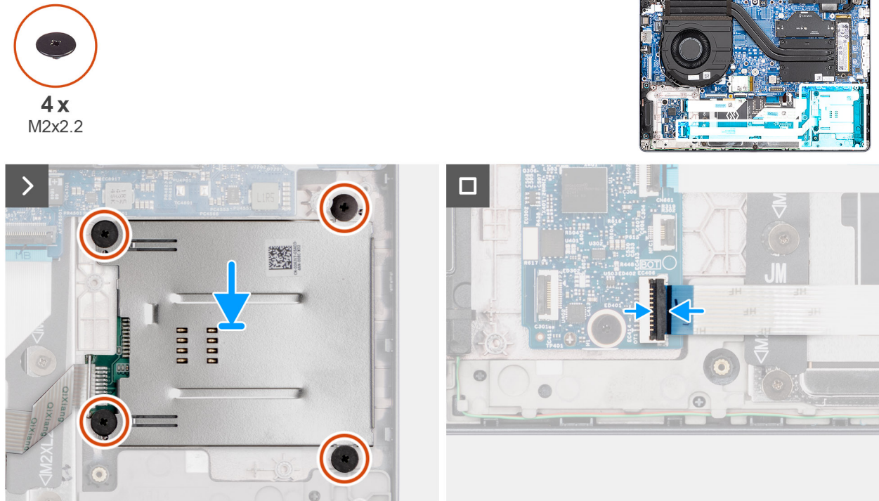
Figura 38. Installing the smart-card reader
