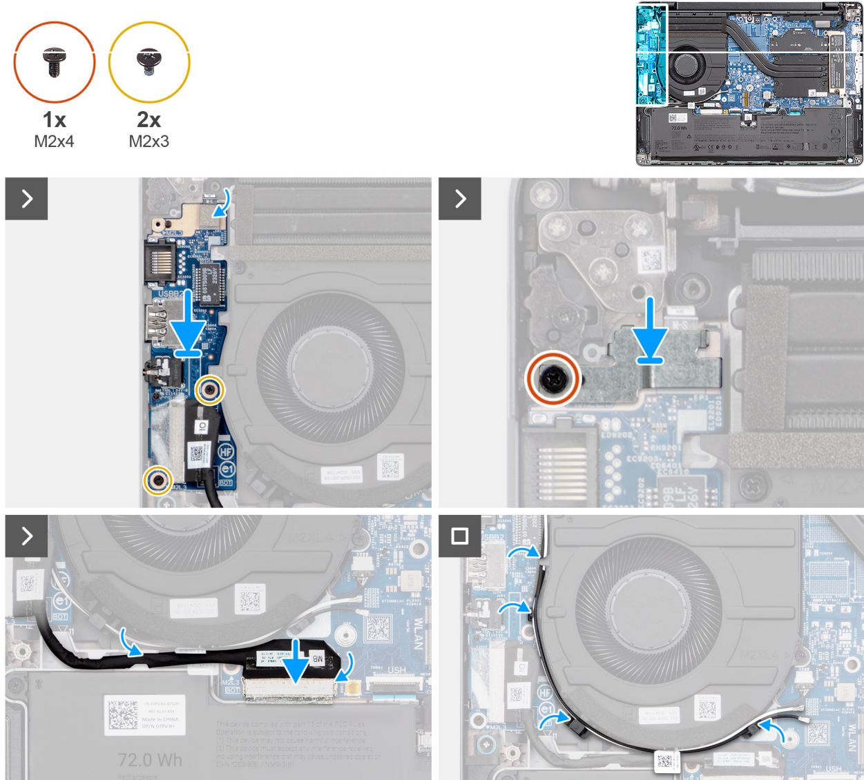
Figura 44. Installing the I/O board
