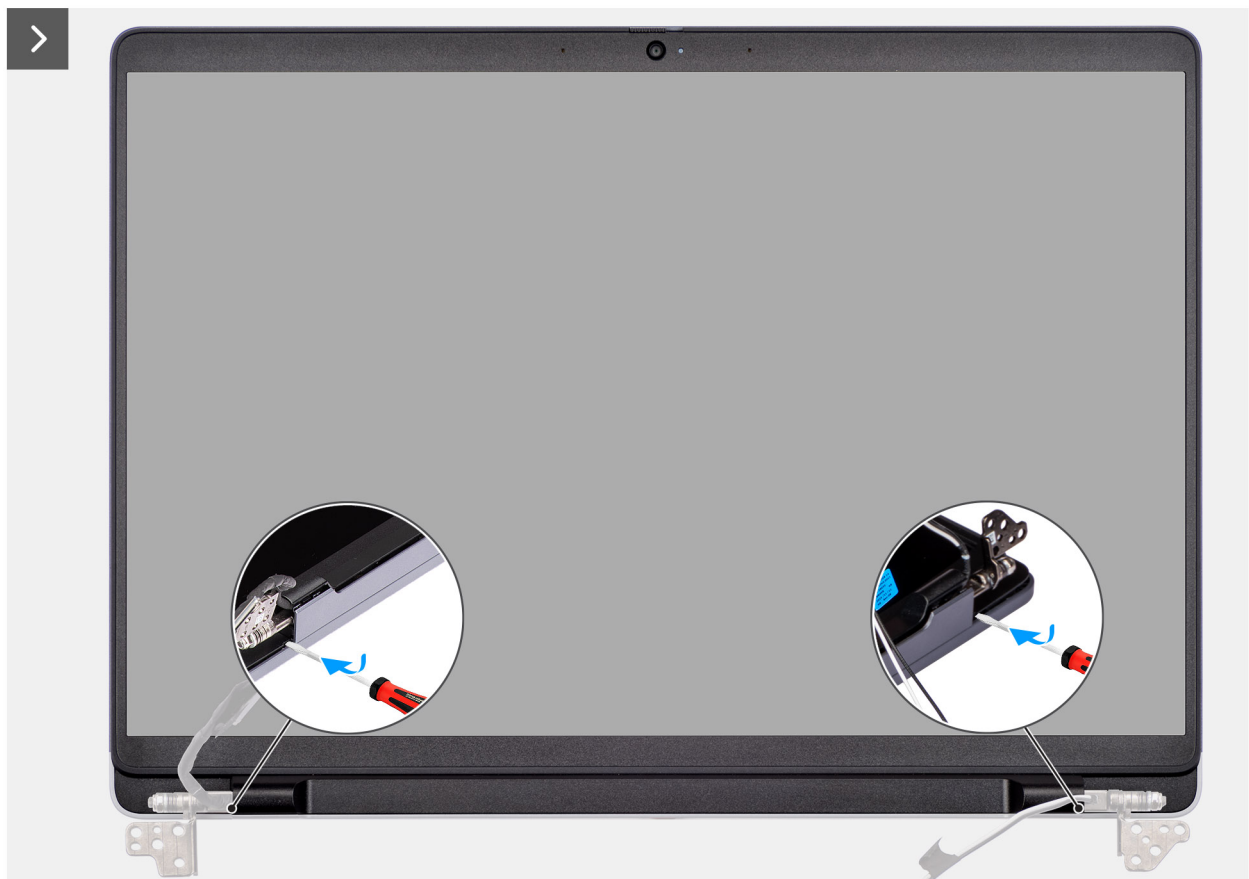
Figura 52. Removing the display bezel
