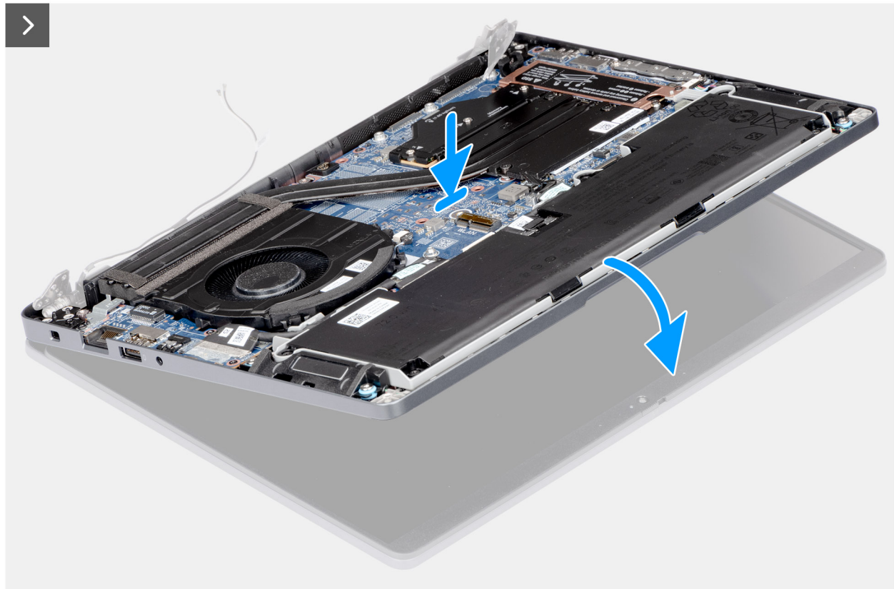
Figura 50. Installing the display assembly
