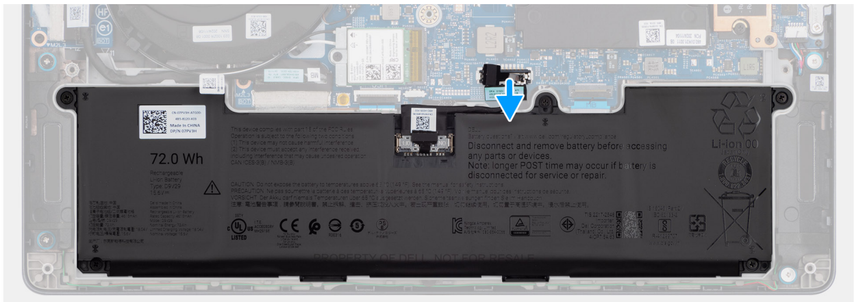
Figura 13. Removing the battery cable
