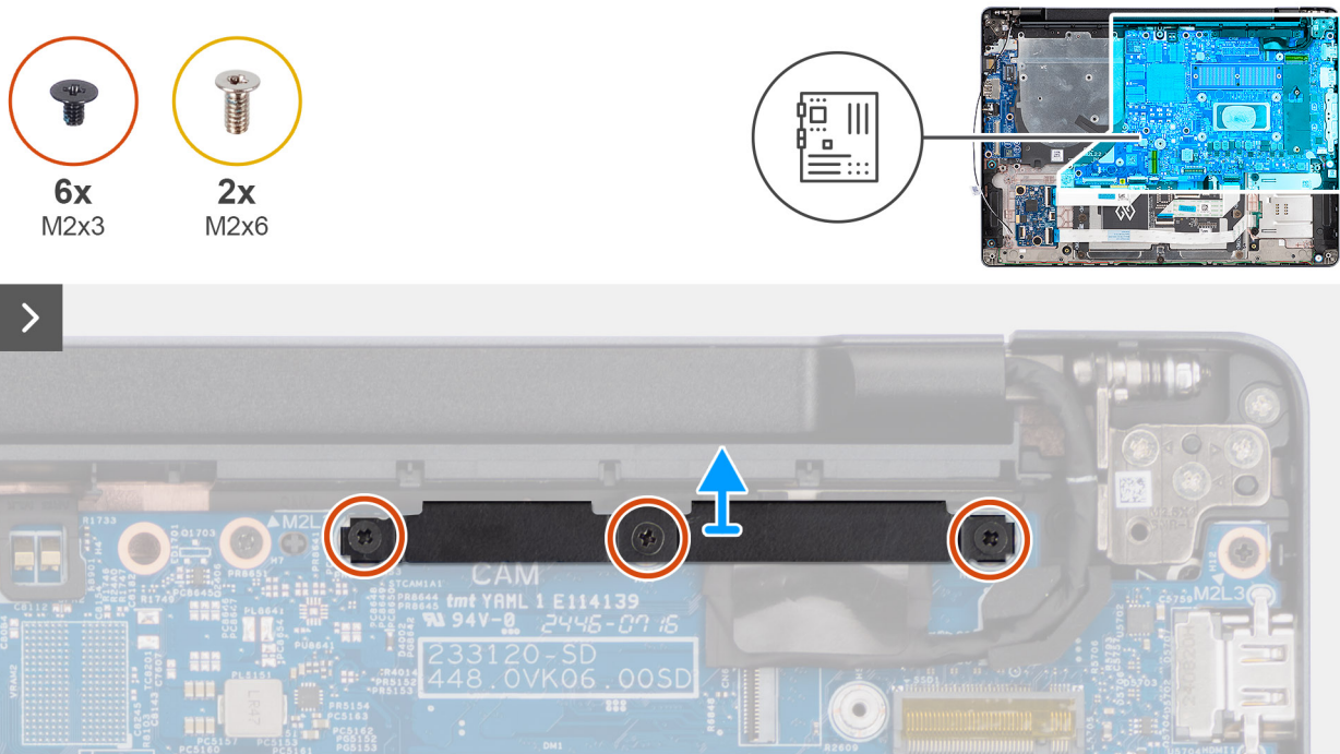
Figura 75. Removing the system board
