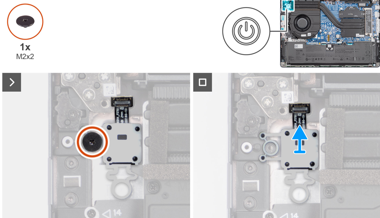
Figura 45. Removing the power button
