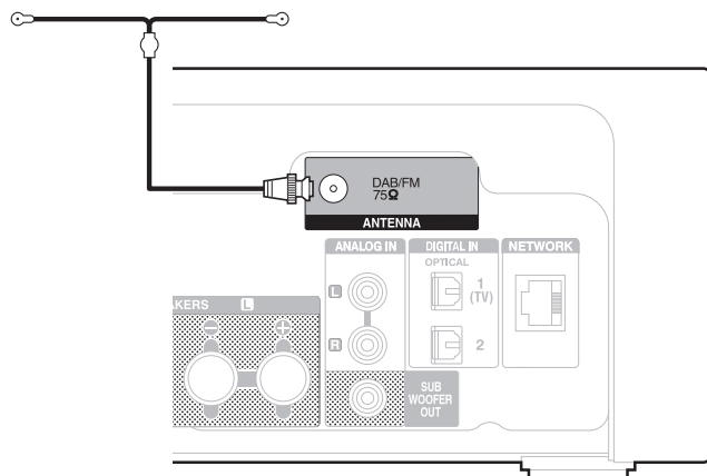
DAB/FM indoor antenna (supplied)
