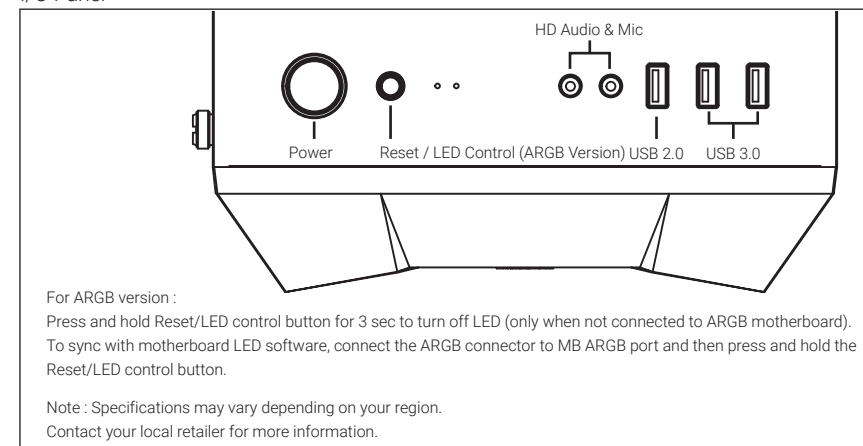
I/O Panel
