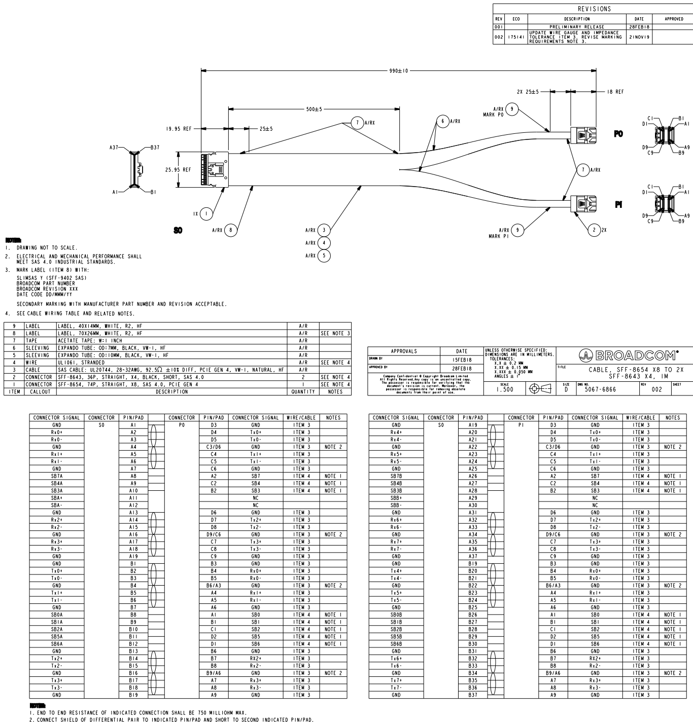
Figure 17: Cable 05-60003-00 Drawing and Pinout
