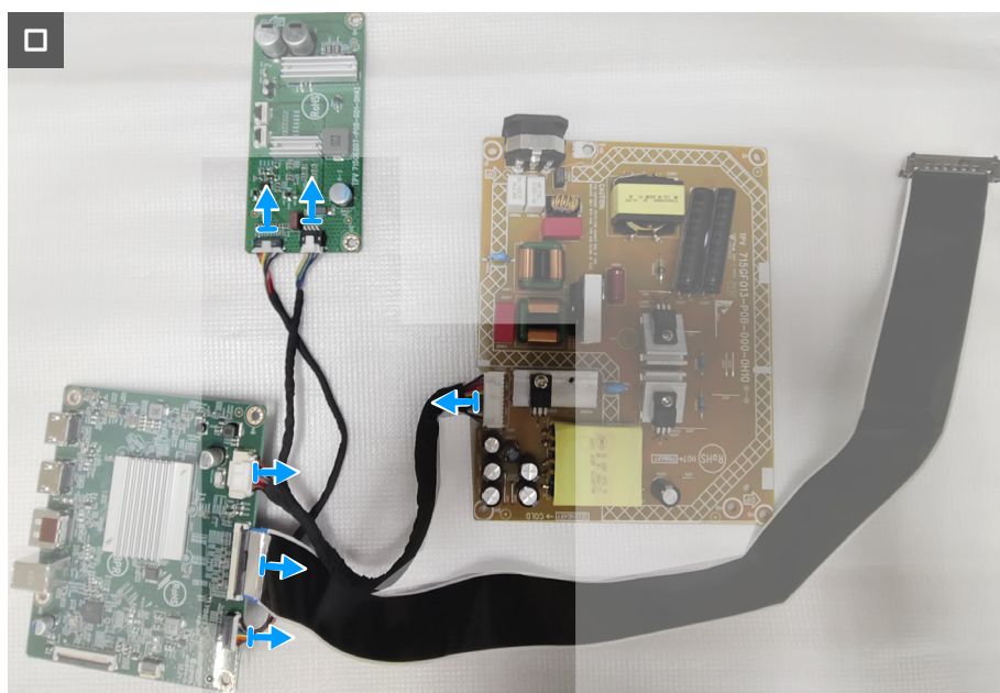
Figure 32. Removing the system board and power board
