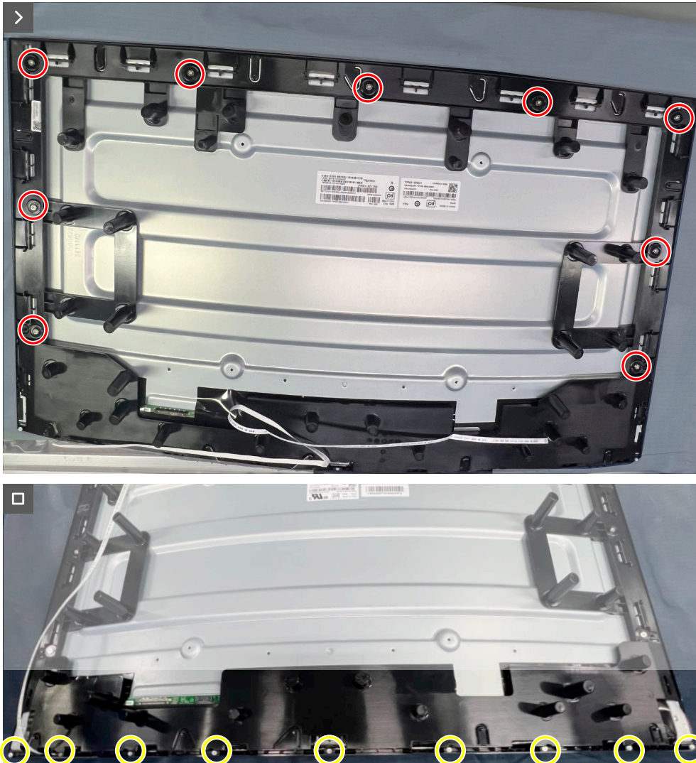
Figure 37. Installing the middle frame
