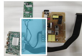
Figure 31. Removing the system board and power board
