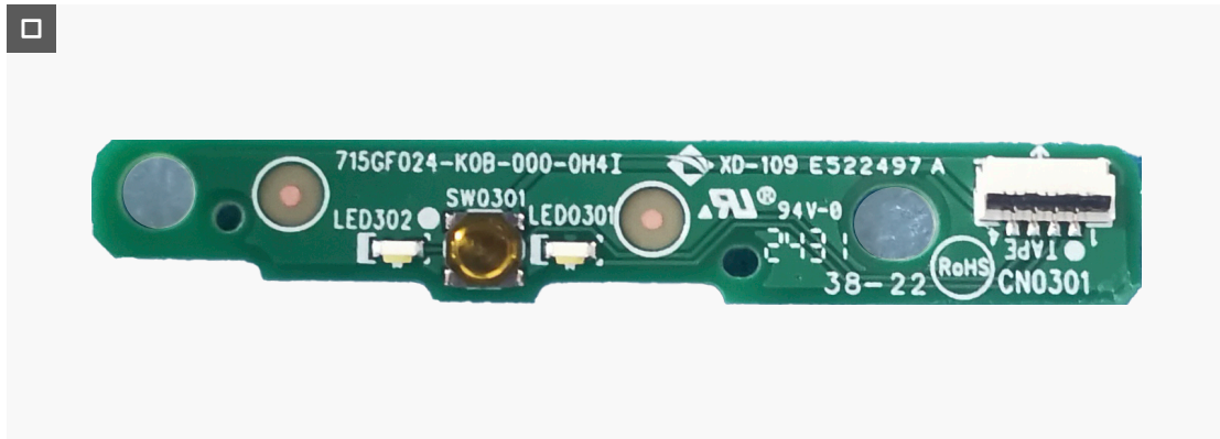
Figure 39. Removing the power-button board
