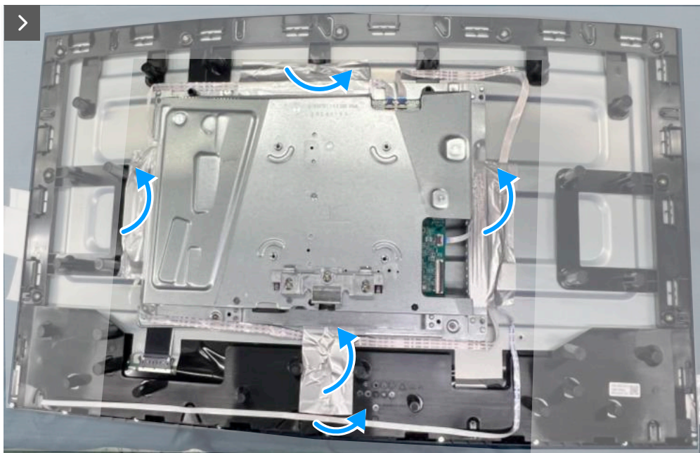
Figure 20. Removing the metal shield
