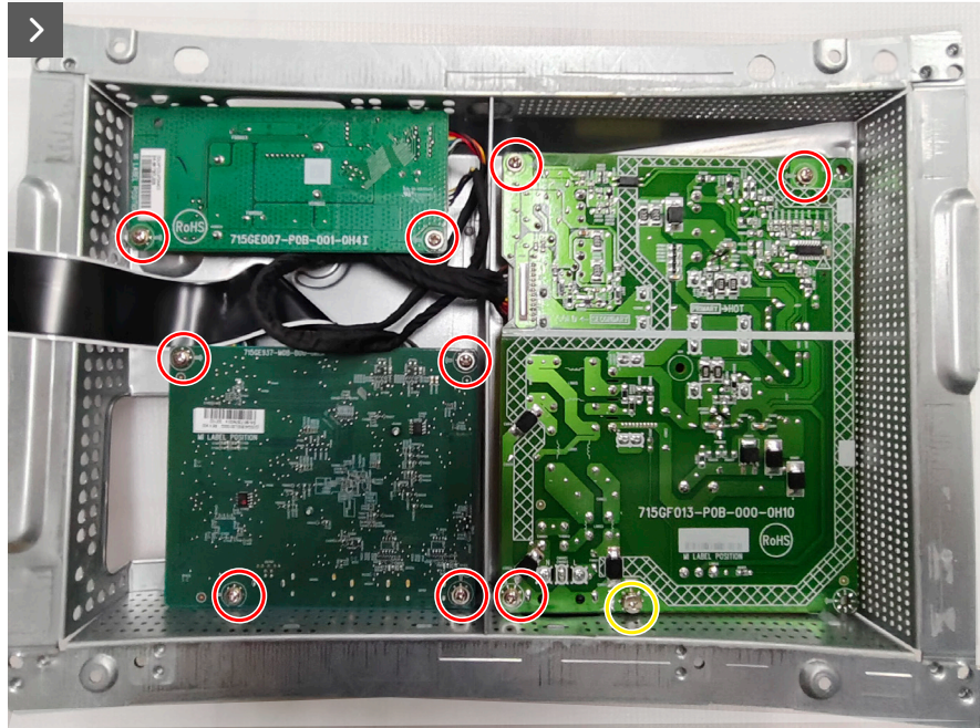
Figure 31. Removing the system board and power board
