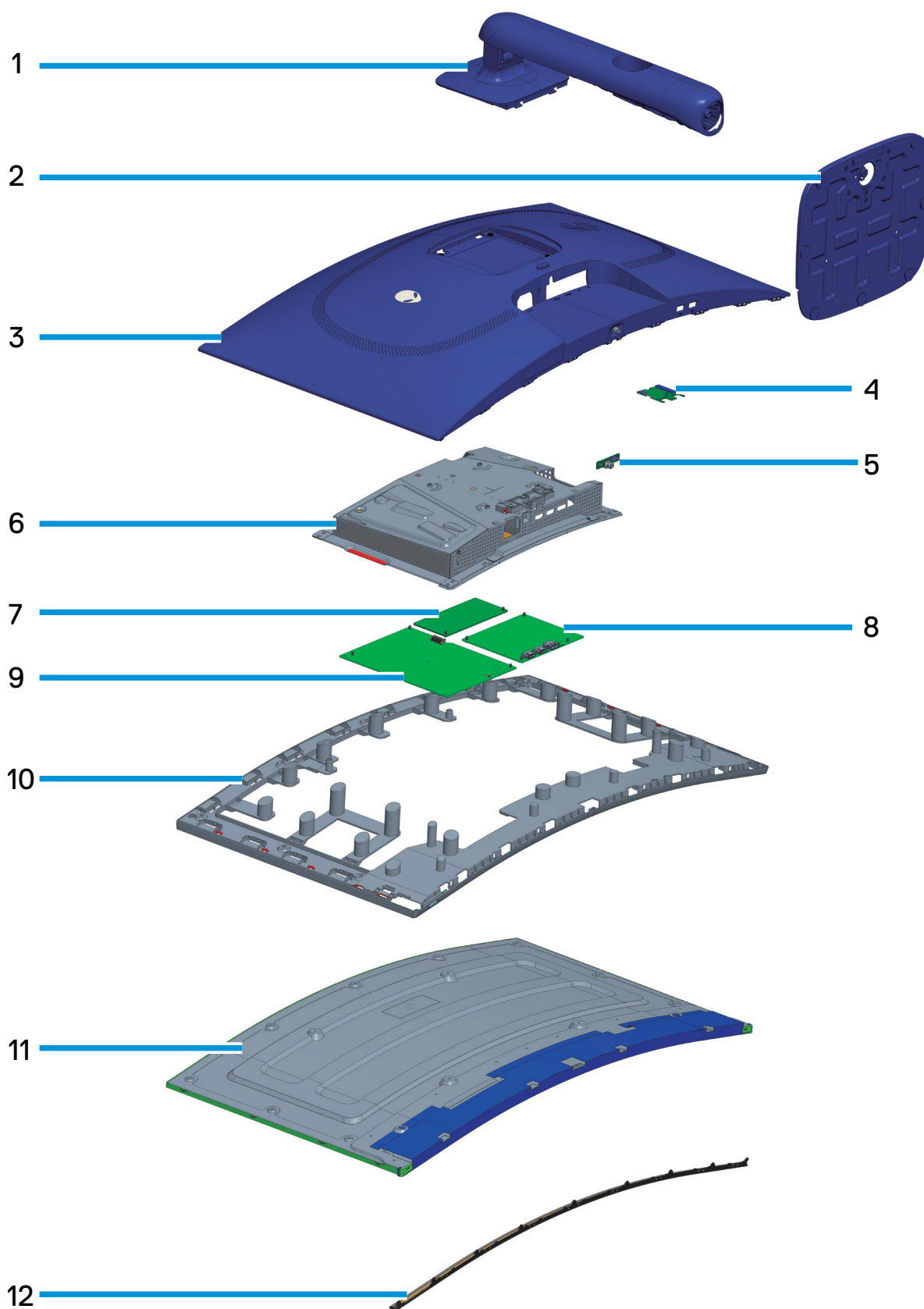
Figure 5. Major components of AW3225DM
