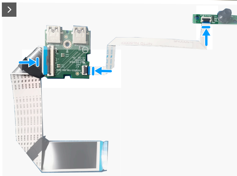
Figure 43. Installing the I/O board and joystick-button board
