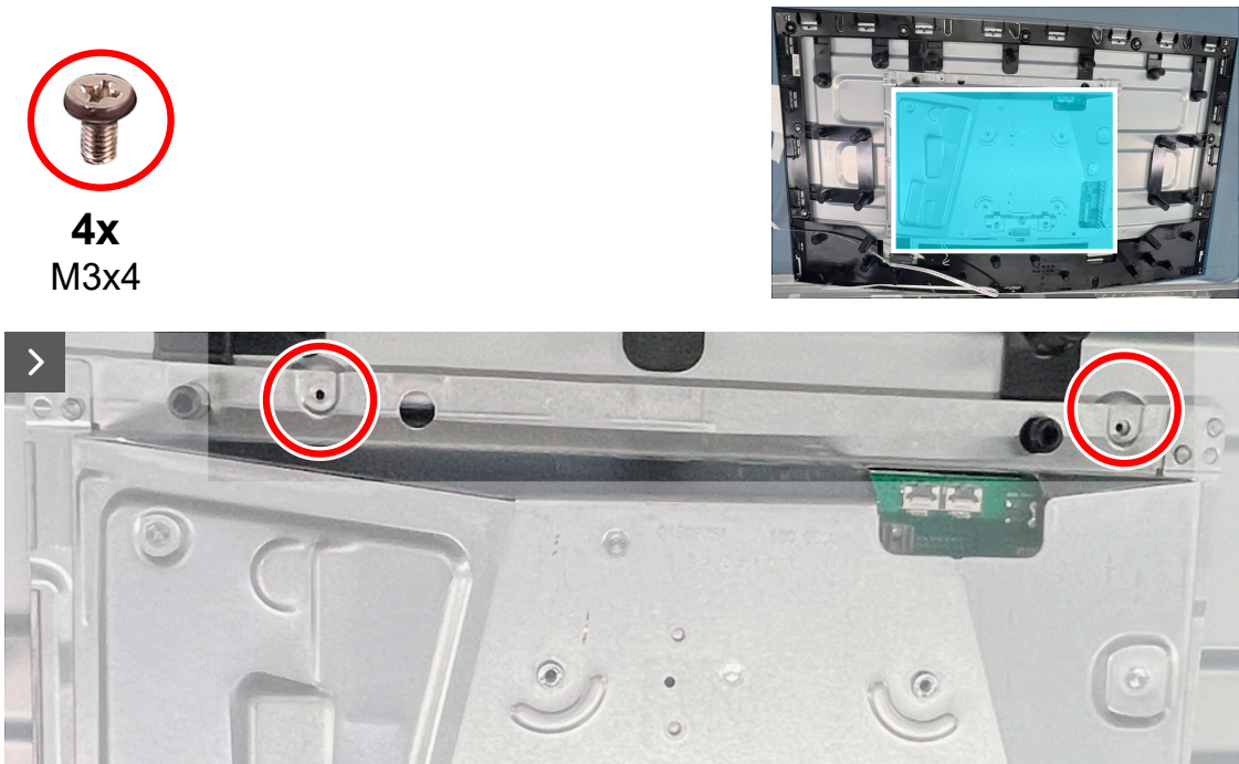
Figure 22. Removing the metal shield
