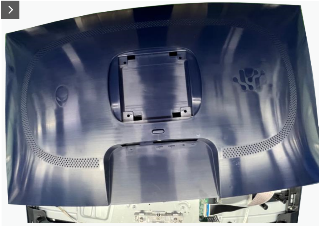
Figure 15. Removing the back cover
