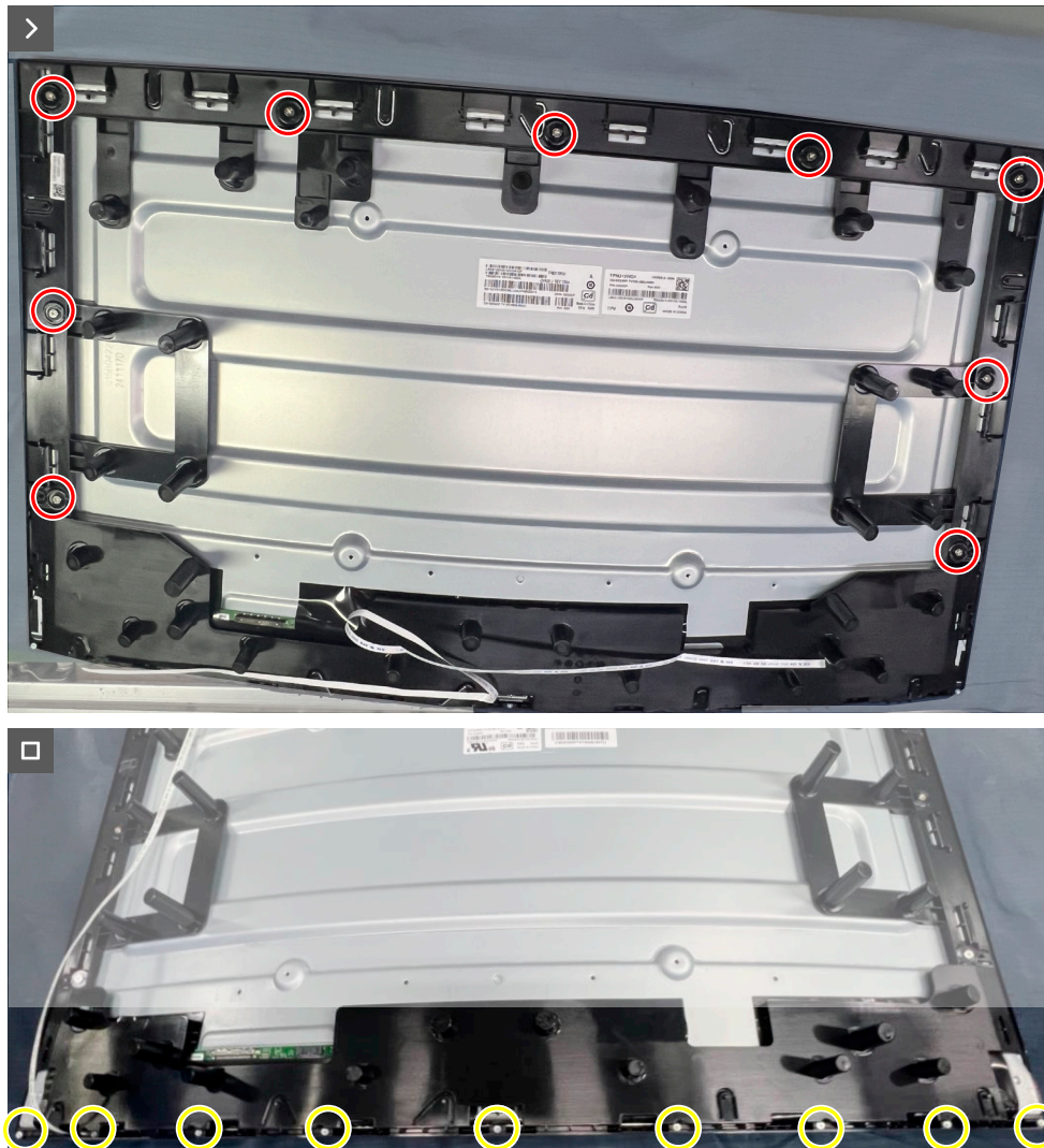
Figure 36. Removing the middle frame
