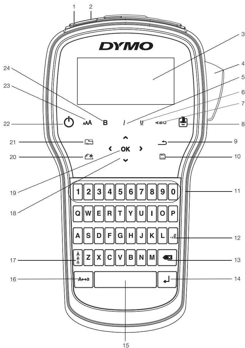
Figur 1 LabelManager 280 merkemaskin
