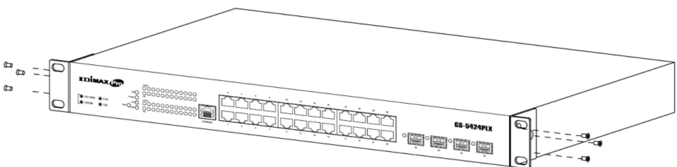
Figure 5 - Bracket Installation
