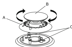
Fig. 10: positioning of the series III burner
