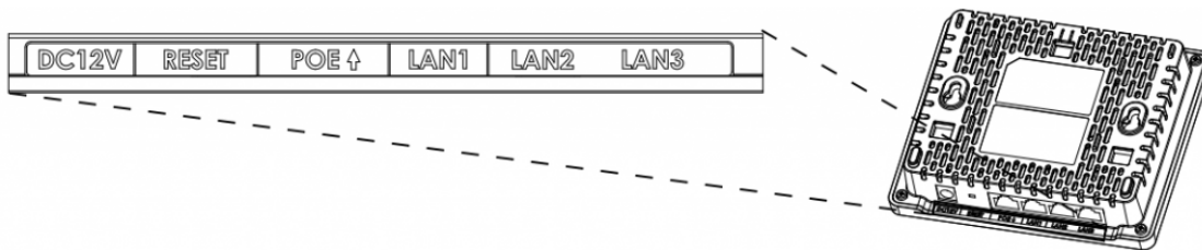
GWN7602 Ports
