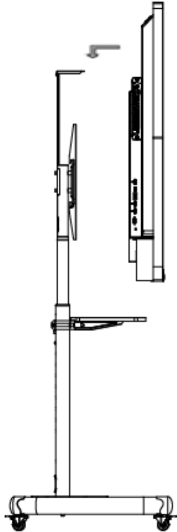
Figure 3-6 Mobile Mounting
