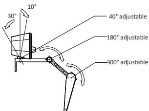
Figure 2-1 Angle Adjustment
