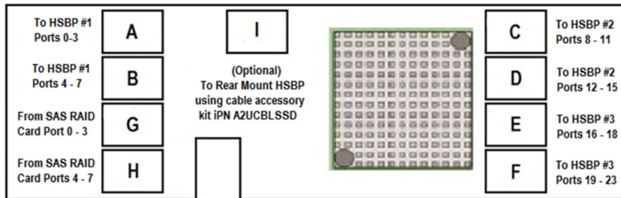
Figure 26. SAS Expander RES3TV360 Port Mapping
